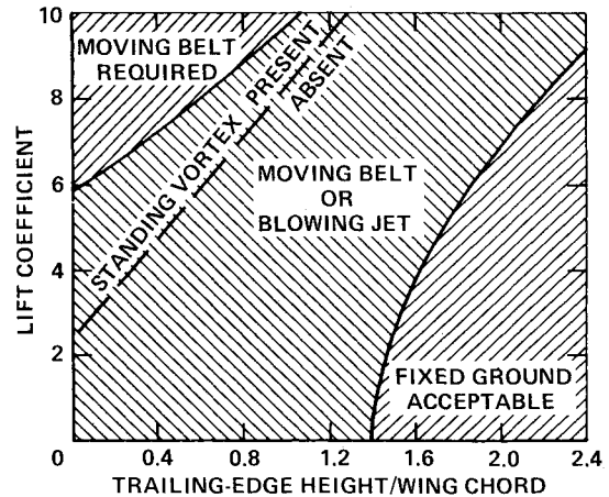
Fig. 6 Test ranges for fixed ground, blowing jet, and moving belt.
