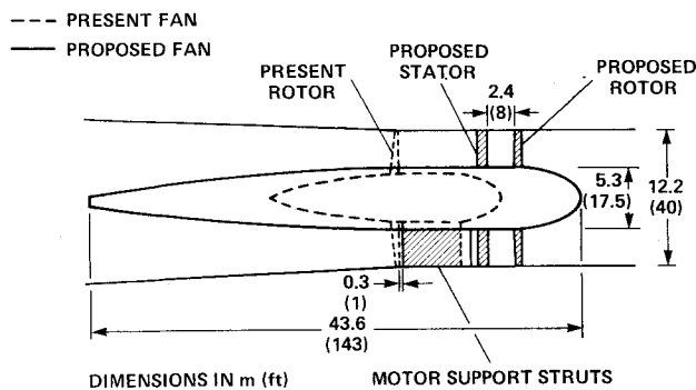
Fig. 8 Change in drive system geometry.
