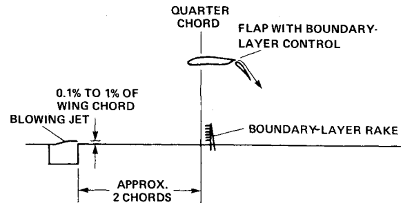
Fig. 5 Ground-effect testing using floor blowing.
